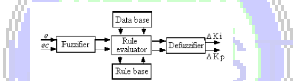
Fig.5 Block diagram of the fuzzy adjustor unit
