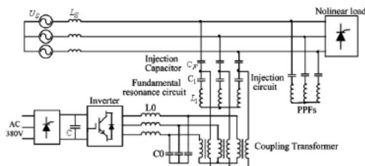
Fig.2 Topology of the novel HAPF
