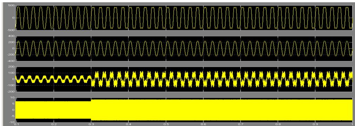
Fig.7 Simulation results of steady-state compensation. (a) Simulation results with the conventional generalized integral controller. (b) Simulation results with the proposed fuzzy controller
