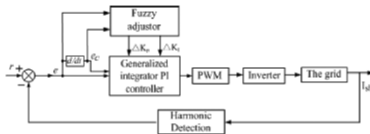
Fig.4 Configuration of the adaptive fuzzy dividing frequency controller
