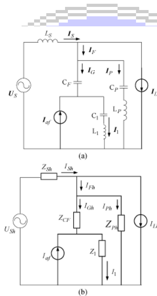
Fig.3 Single-phase equivalent circuit. (a) Single-phase equivalent circuit. (b) Single-phase equivalent circuit with the effect of a harmonic source
