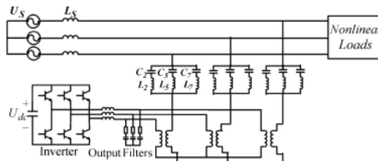
Fig.1 Topology of the shunt hybrid APF
