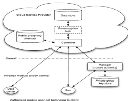
Figure 1: Cloud based application with prediction process.
