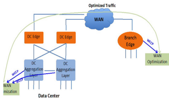
Figure 3: Procedure for the activated processing of the Traffic redundancy in cloud computing.
