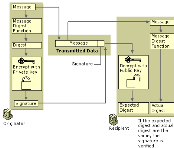
Figure 2: Digital Signature processing application development.
