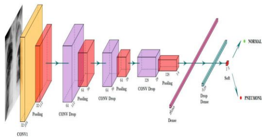
Fig: Overview structure of the proposed lung nodule detection and classification system
